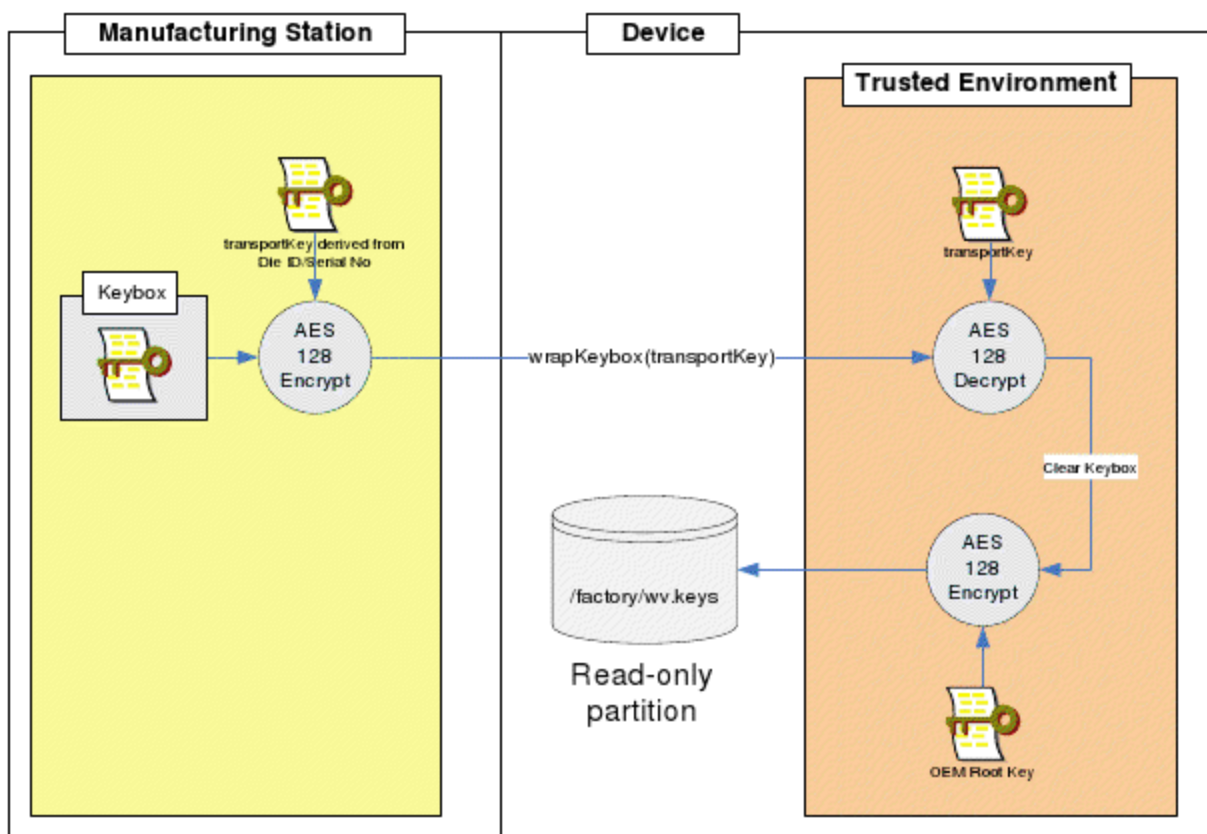
Figure 10. OEMCrypto_WrapKeybox Operation
