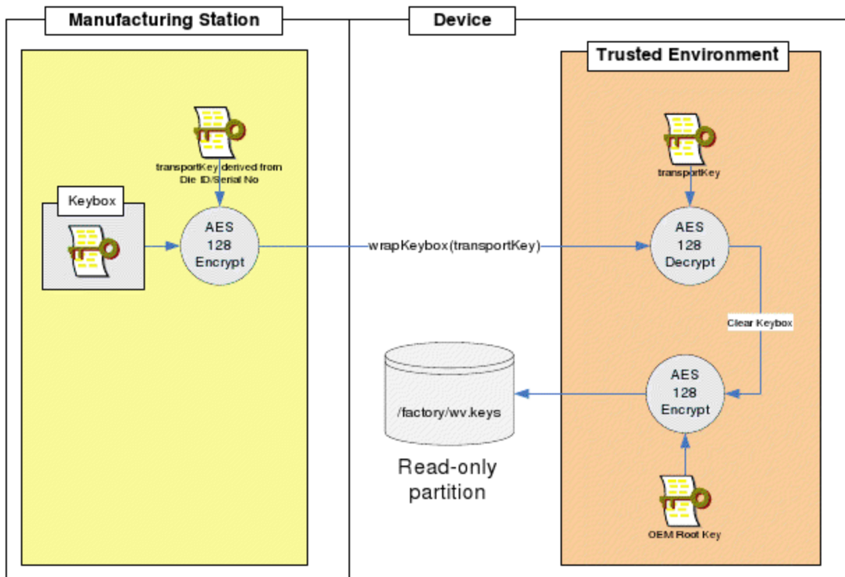
Figure 10. OEMCrypto_WrapKeybox Operation
