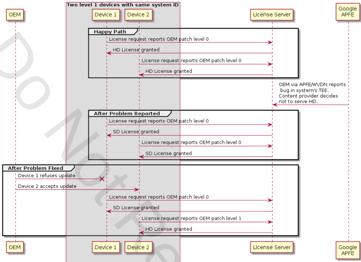
Patch Level Update Sequence Diagram
