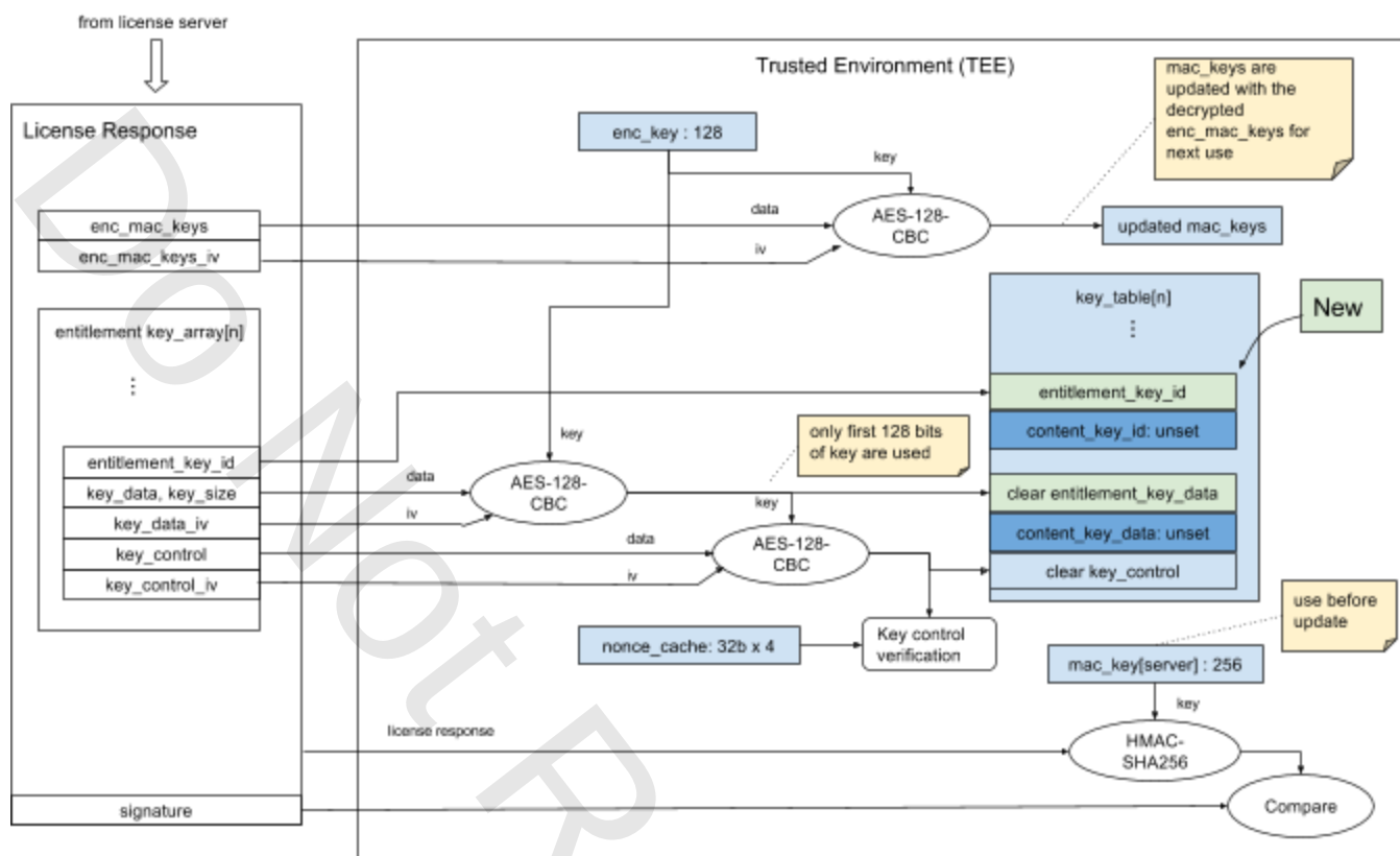
OEMCrypto_LoadKeys() with license_type = OEMCrypto_EntitlementLicense
